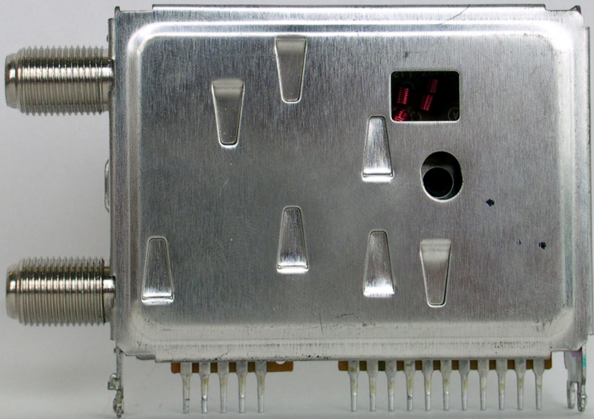
Tuner 2
