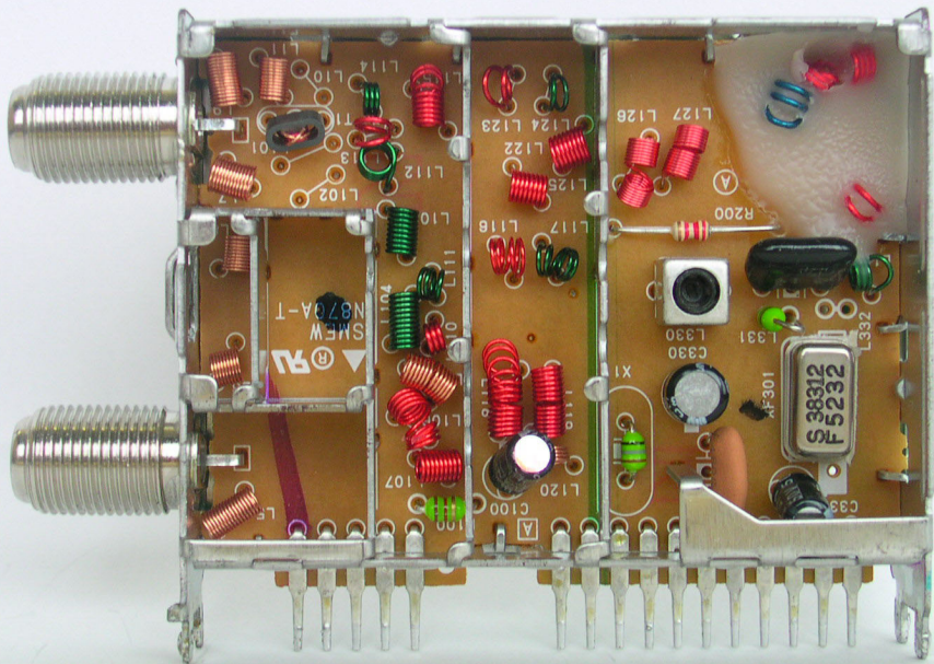
Tuner 3
