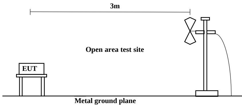
Figure 2. Radiated emission
