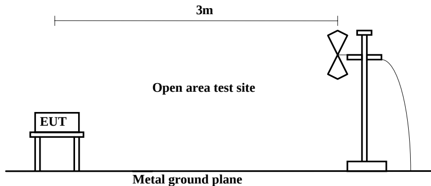
Figure 2. Radiated emission
