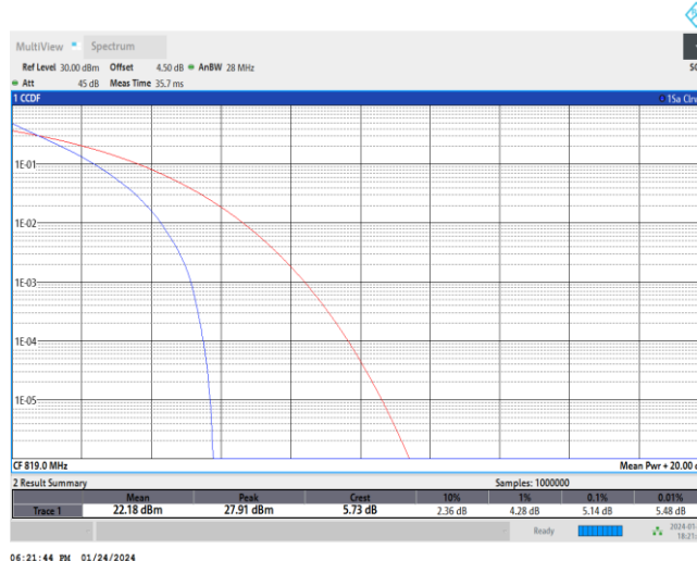
Band26-1.4MHz-QPSK-26740-6RB#0
