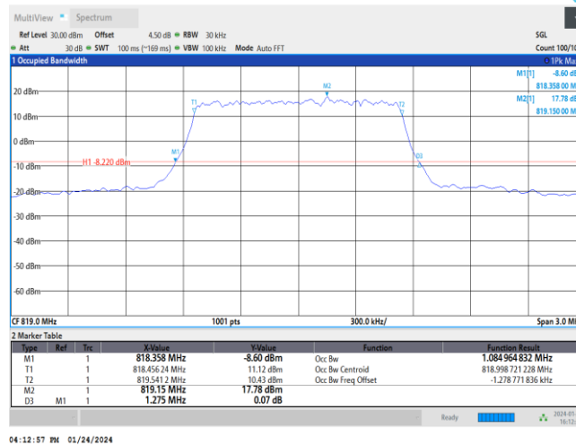
Band26-1.4MHz-16QAM-26740-6RB#0
