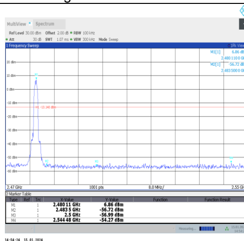
2DH5-Ant1-2480-PASS
