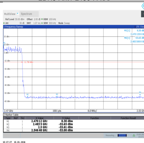
2DH5-Ant1-Hop_2480-PASS
