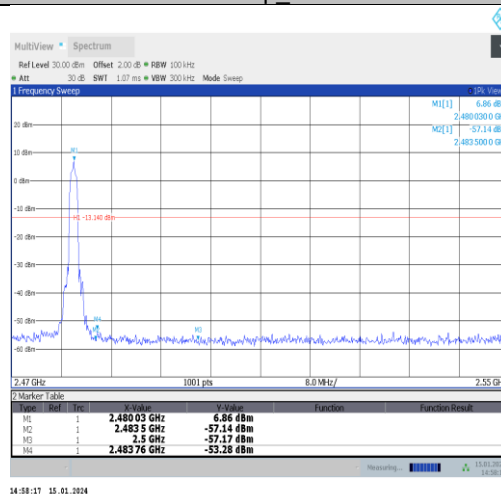
3DH5-Ant1-2480-PASS
