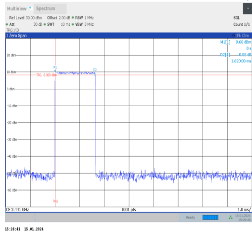
3DH3-Ant1-Hop-PASS
