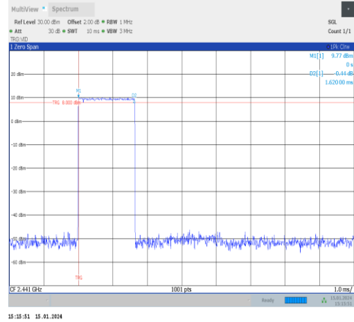
2DH3-Ant1-Hop-PASS
