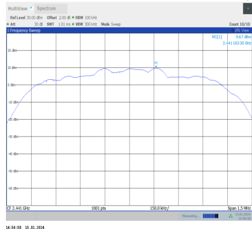
3DH5-Ant1-2441-0~Reference-PASS
