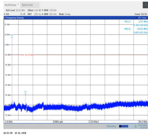
2DH5-Ant1-2402-1000~26500-PASS
