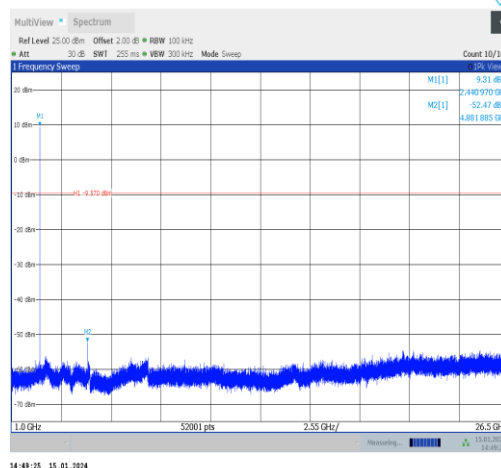
DH5-Ant1-2441-1000~26500-PASS
