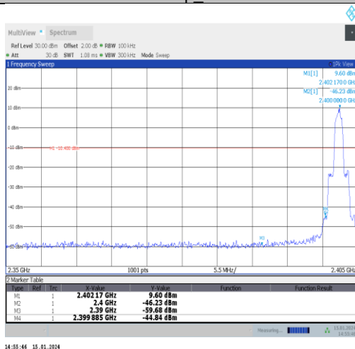
3DH5-Ant1-2402-PASS
