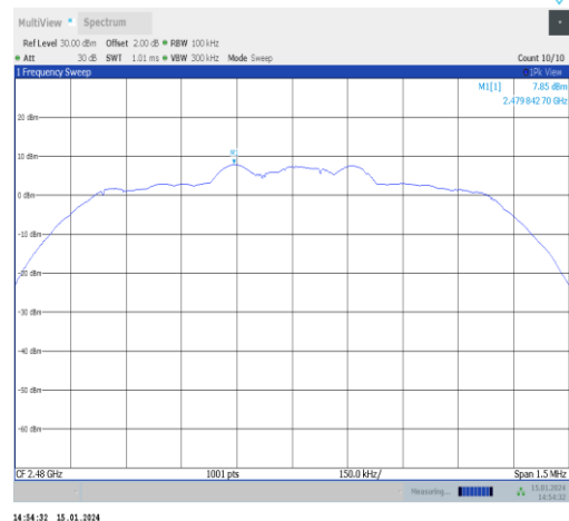
2DH5-Ant1-2480-0~Reference-PASS
