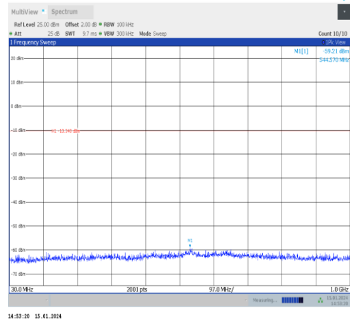
2DH5-Ant1-2441-30~1000-PASS
