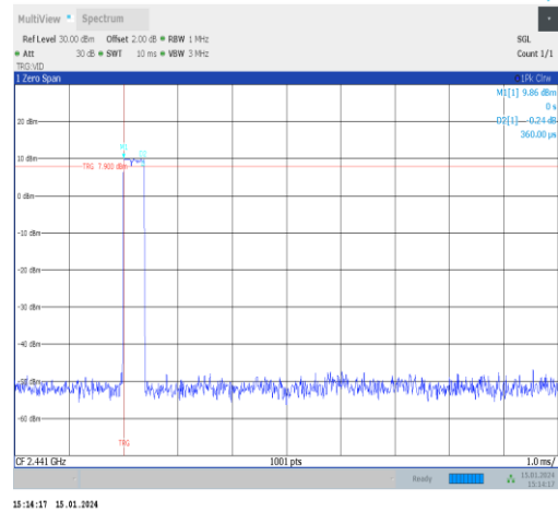
2DH1-Ant1-Hop-PASS
