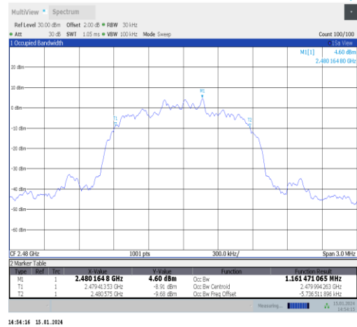
2DH5-Ant1-2480
