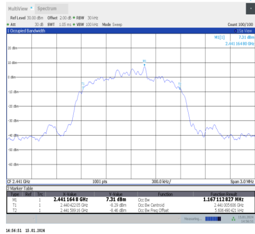
3DH5-Ant1-2441
