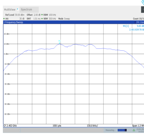
2DH5-Ant1-2402-0~Reference-PASS
