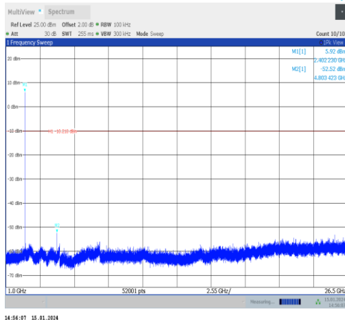
3DH5-Ant1-2402-1000~26500-PASS
