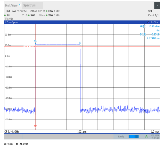
DH5-Ant1-Hop-PASS
