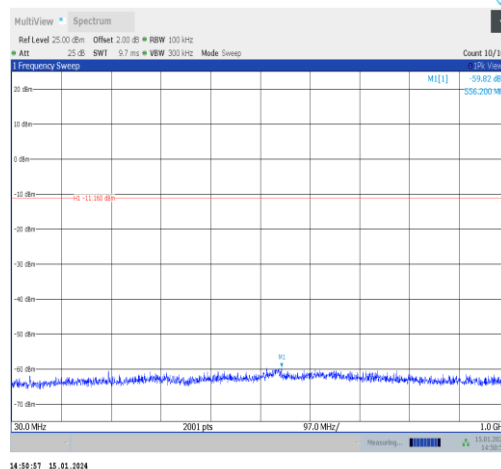
DH5-Ant1-2480-30~1000-PASS
