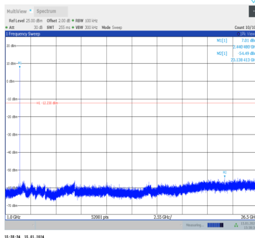
BLE_1M-Ant1-2440-1000~26500-PASS
