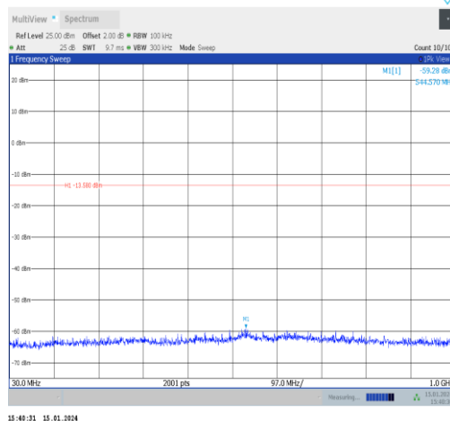
BLE_1M-Ant1-2480-30~1000-PASS
