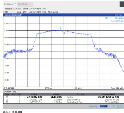
11n40SISO-Ant1-2452
