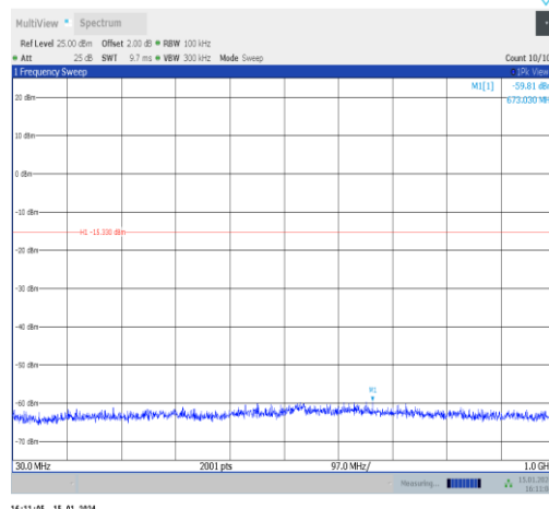
11n20SISO-Ant1-2462-30~1000-PASS
