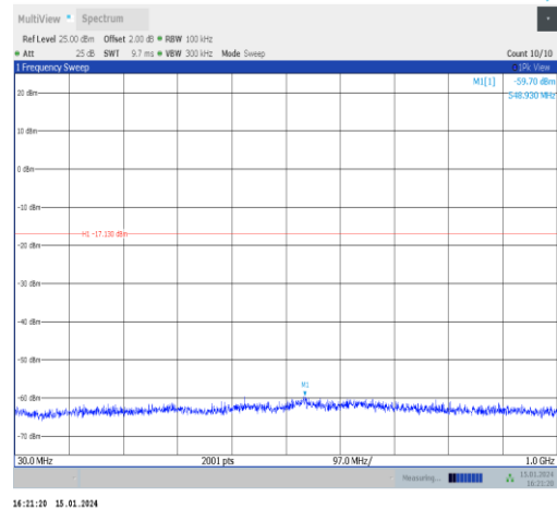
11n40SISO-Ant1-2437-30~1000-PASS
