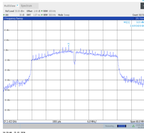
11n40SISO-Ant1-2422-0~Reference-PASS
