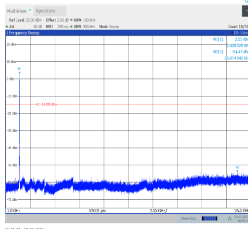
11n20SISO-Ant1-2437-1000~26500-PASS
