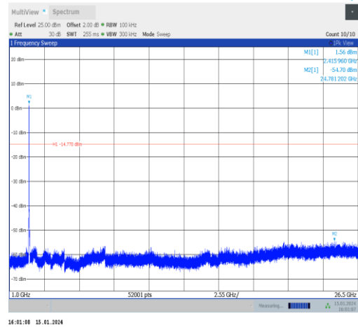
11g-Ant1-2412-1000~26500-PASS
