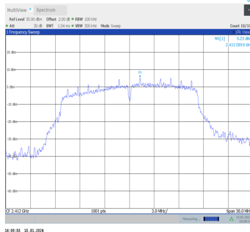
11g-Ant1-2412-0~Reference-PASS
