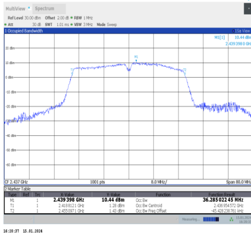
11n40SISO-Ant1-2437
