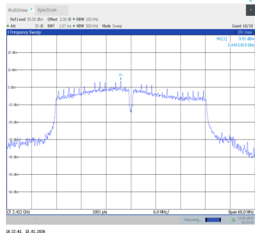
11n40SISO-Ant1-2452-0~Reference-PASS
