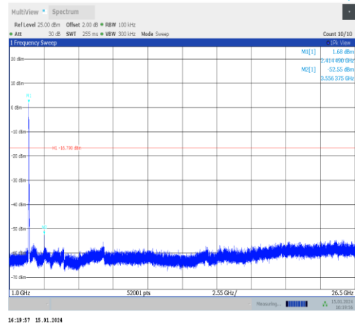
11n40SISO-Ant1-2422-1000~26500-PASS
