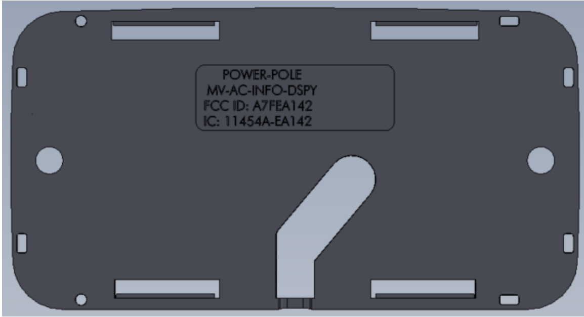
Bottom View of EA142 Housing
