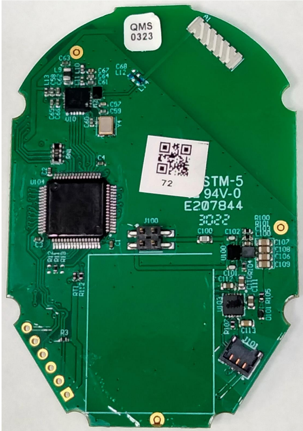
Bottom View of EA131
