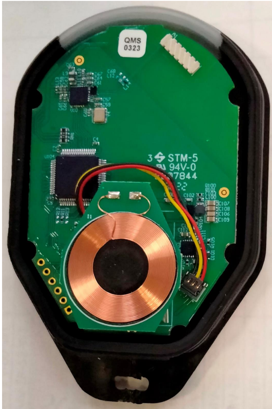
Bottom View of EA131 (In Unit)
