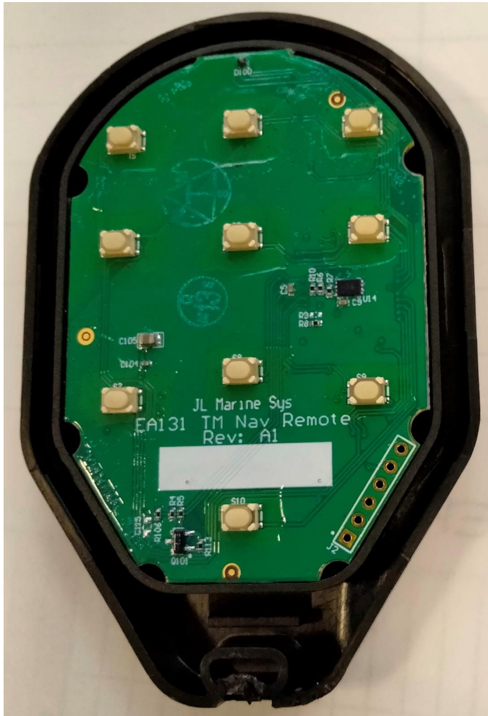
Top View of EA131 (In Unit)
