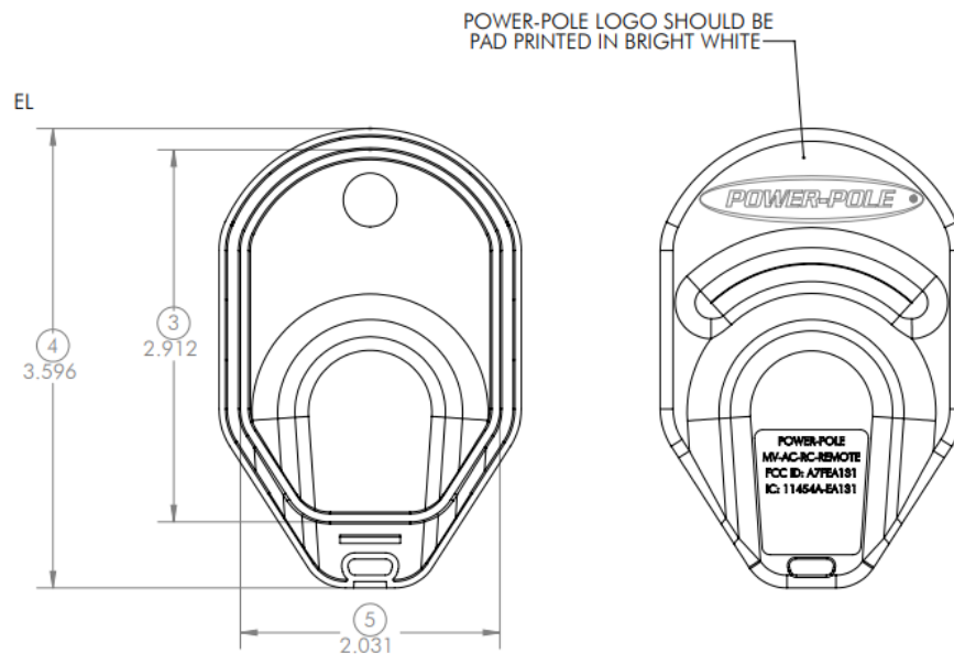
Drawing of EA131 Back Case
