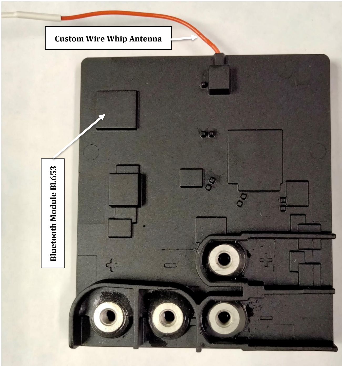
Top View of EA087 (In Molding)
