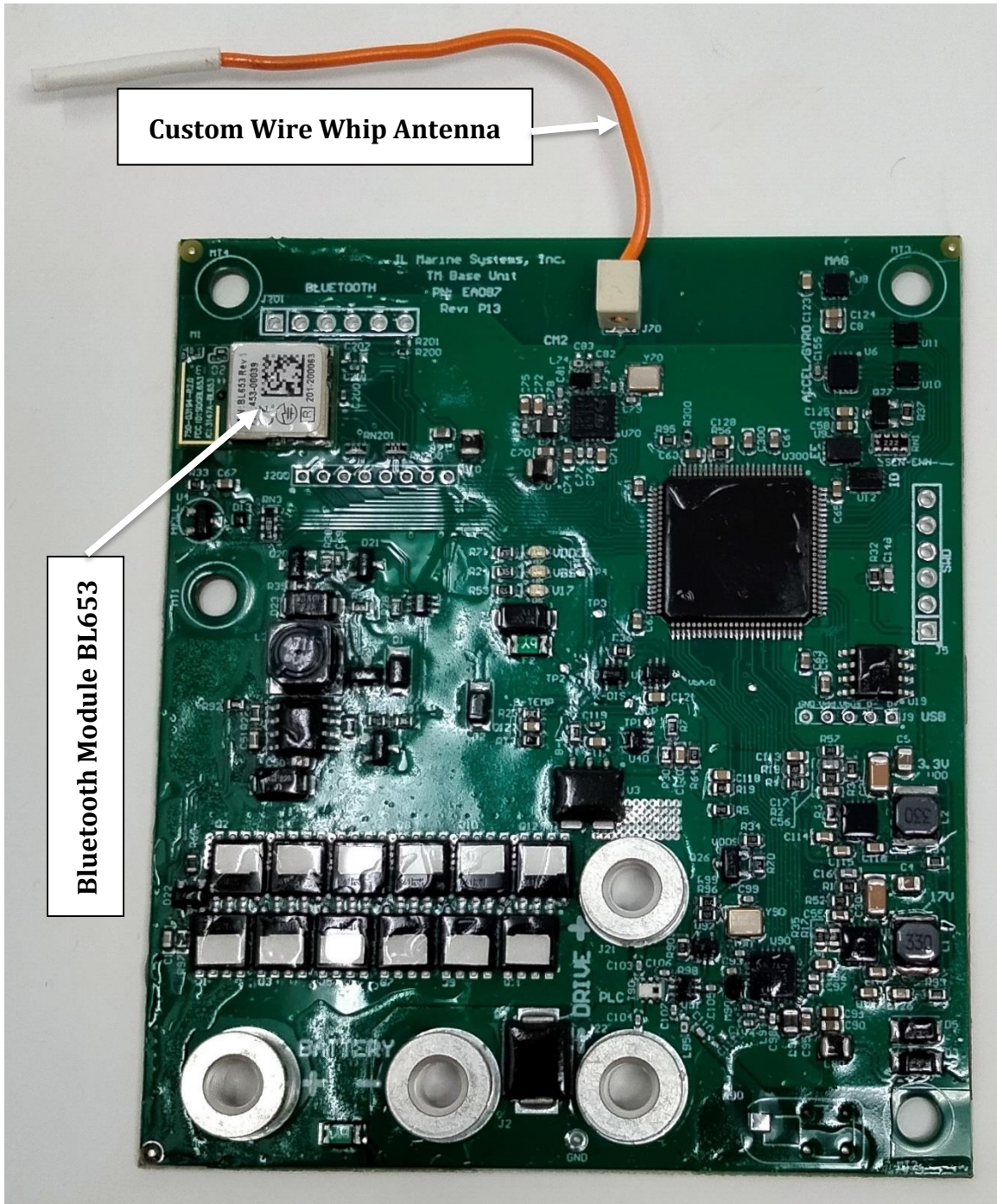
Top View of EA087
