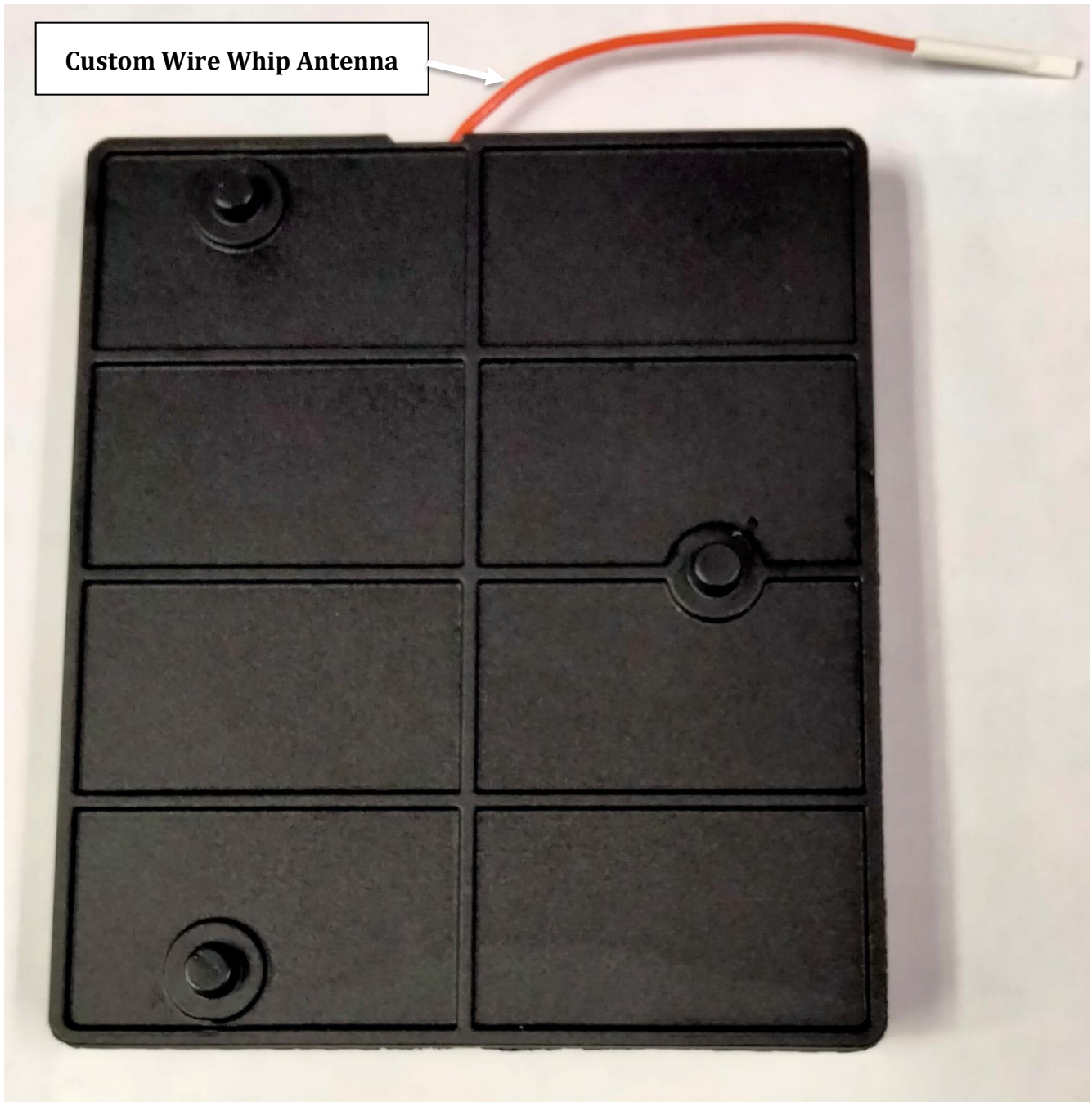
Bottom View of EA087 (In Molding)
