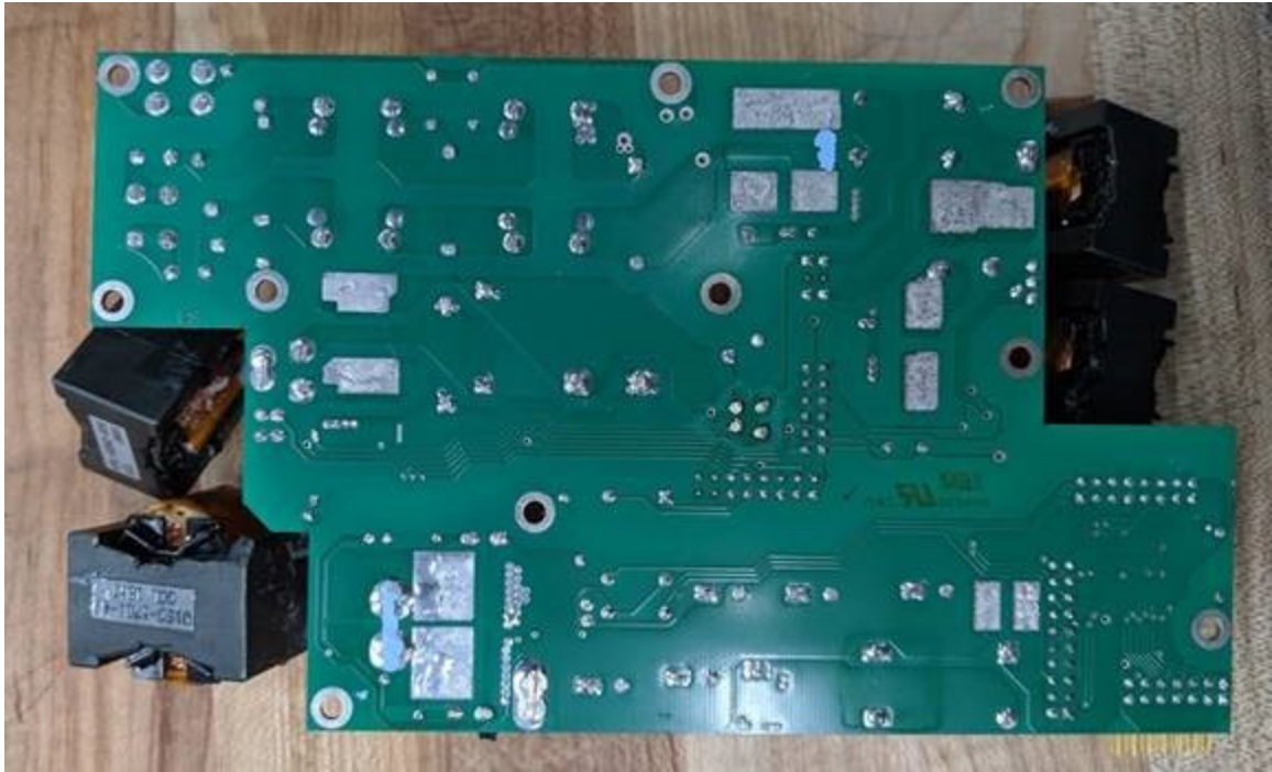
AC BOARD – BOTTOM VIEW
