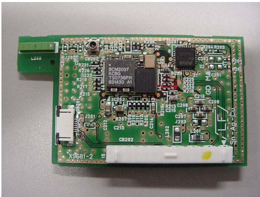
RF Part
