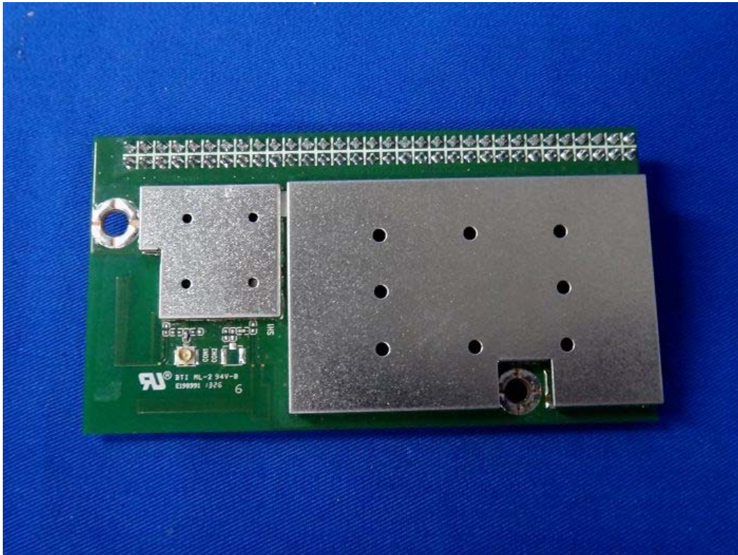
(1) EUT Photo (SDRAM / ESMT)
