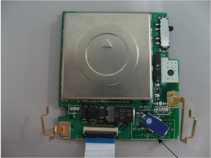
With Shield
