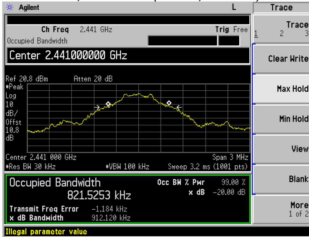
20 dB Bandwidth, Middle Channel (2441 MHz, GFSK Mode)
