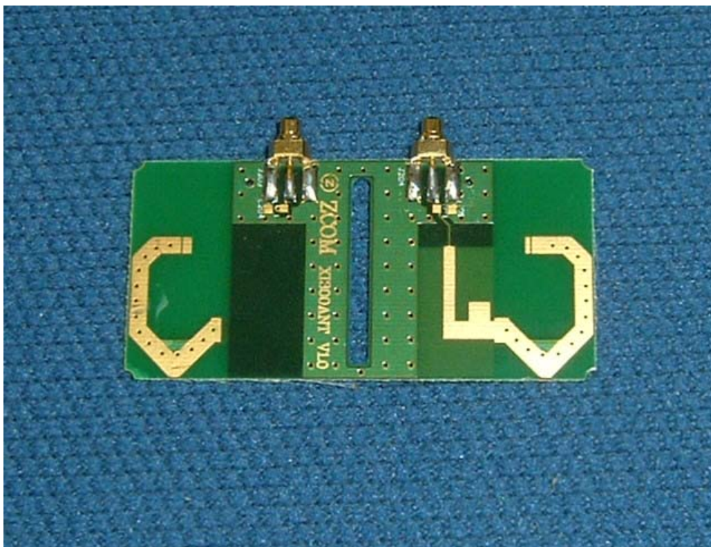
Pattern Antenna (4λ) front
