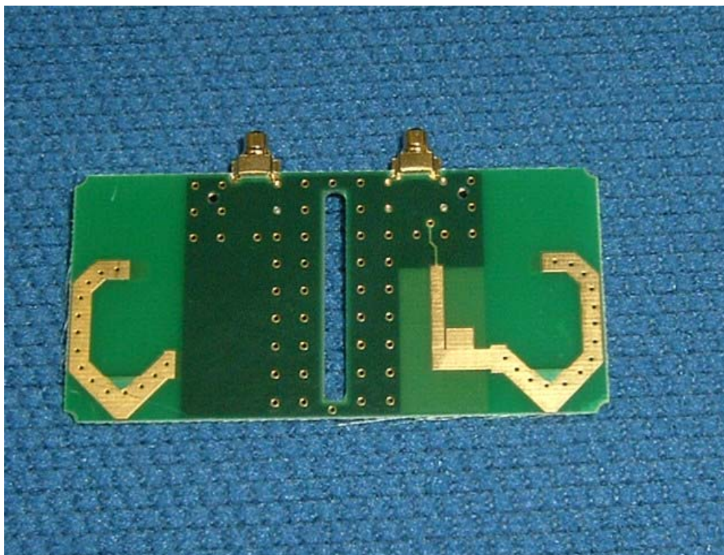
Pattern Antenna (4λ) back
