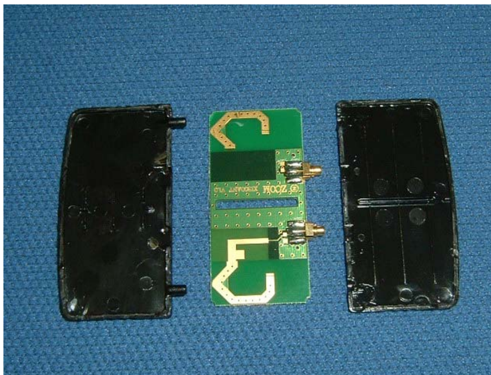
Pattern Antenna (4λ) with cover
