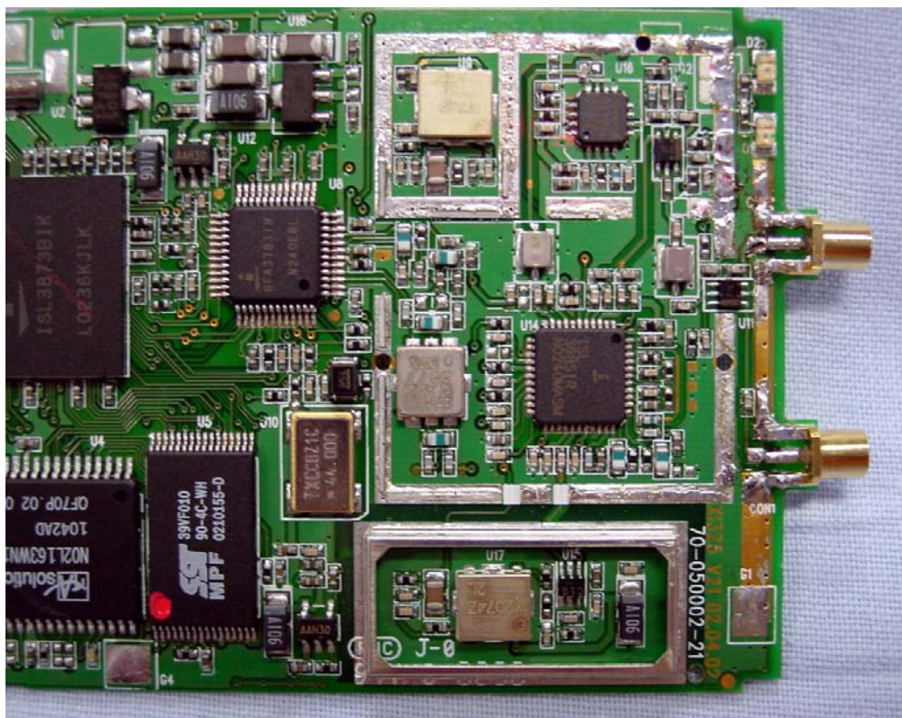
RF PWB Side (Close up)
