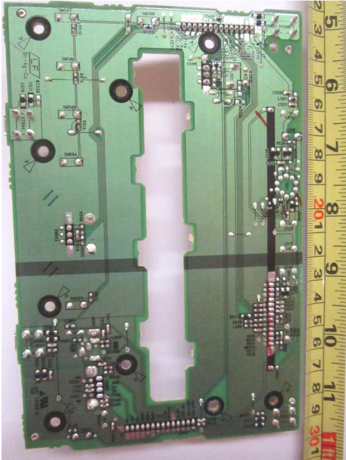
LCD Display PCB Trace Side
