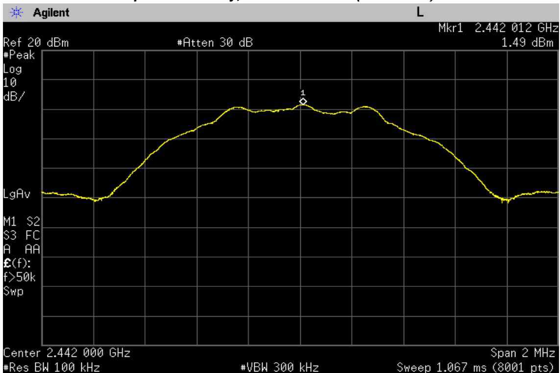
Reference Power Spectral Density, Middle Channel (2 442 MHz)
