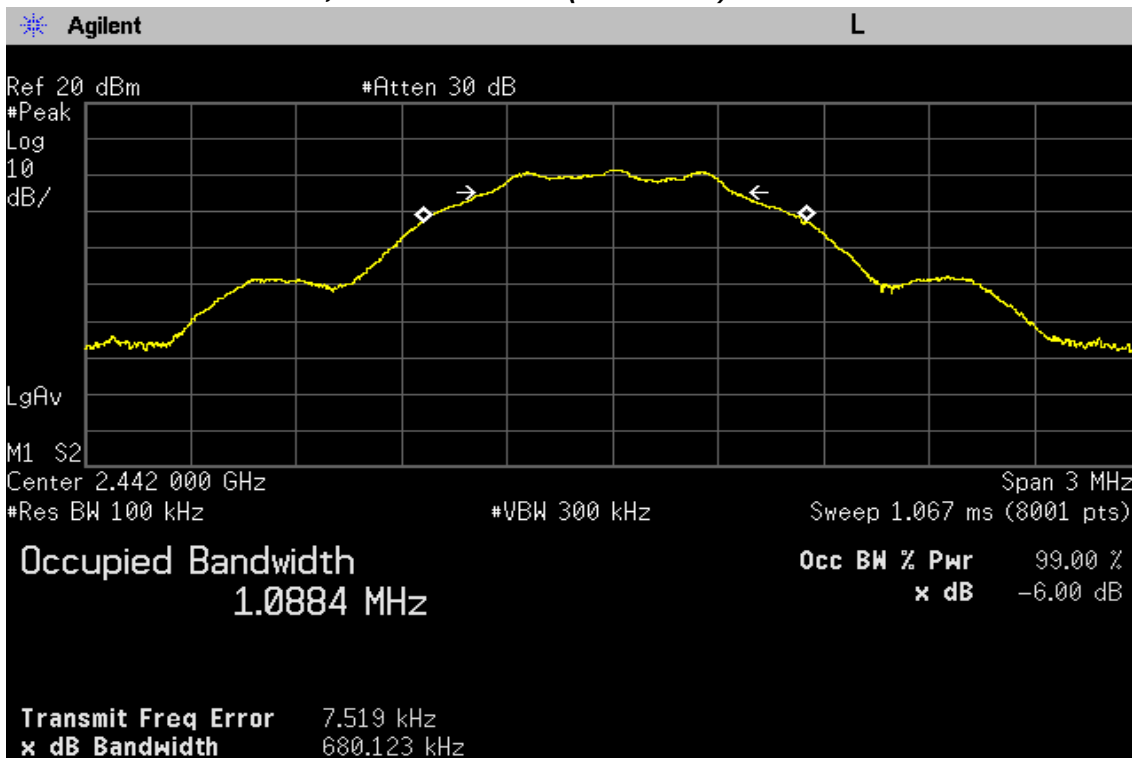
6 dB & 99% Bandwidth, Middle Channel (2 442 MHz)
