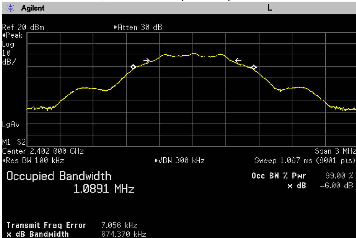
6 dB & 99% Bandwidth, Lowest Channel (2 402 MHz)
