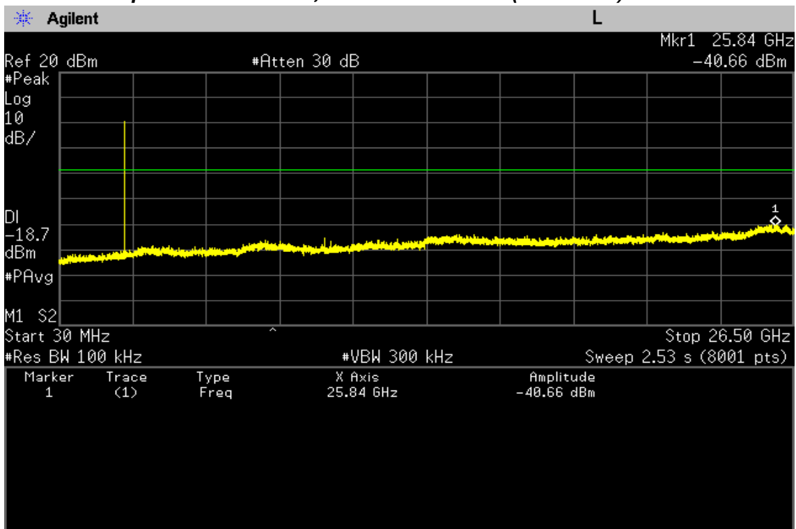
Conducted Spurious Emissions, 30 MHz ~ 26.5 GHz (2 402 MHz)
