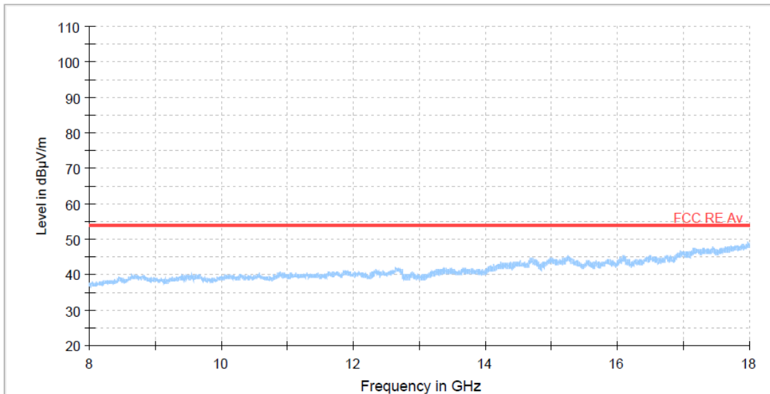
Lowest channel : 8 GHz to 18 GHz_ Average
