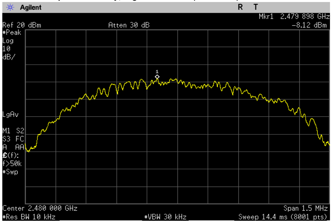
Peak Power Spectral Density, Highest Channel (2 480 MHz)
