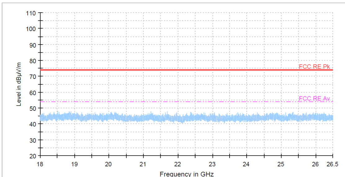
Lowest channel : 18 GHz to 26.5 GHz_ Peak
