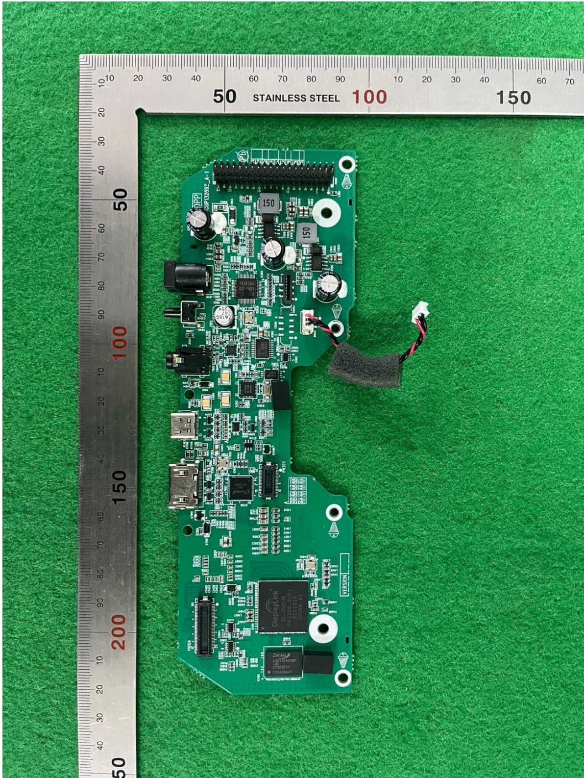
Front View of JACK board
