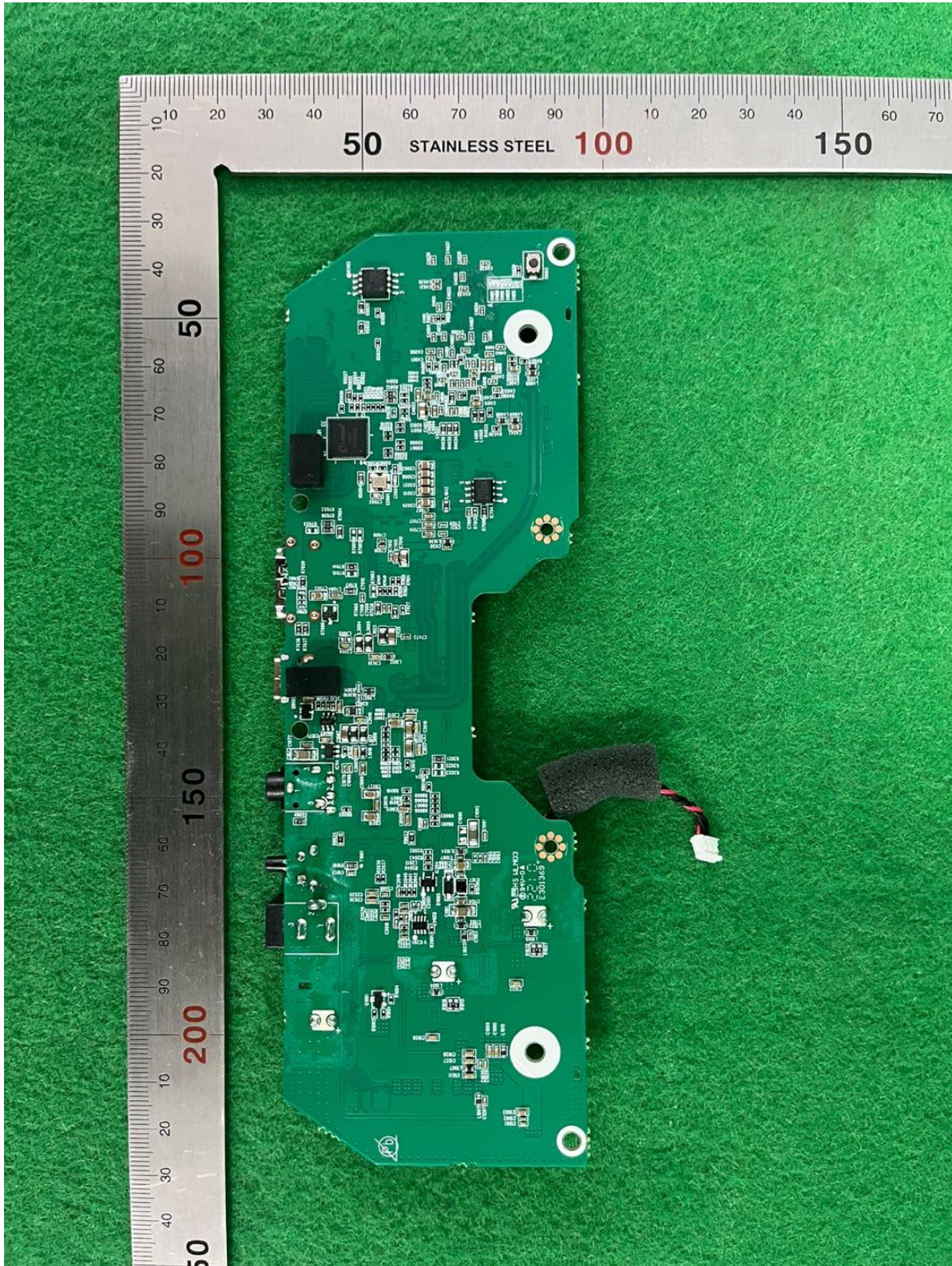
Rear View of JACK board
