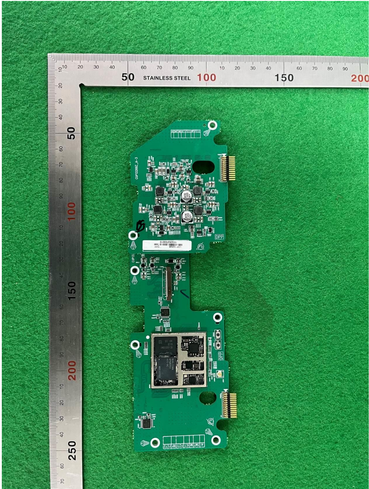
View of Main board Shield can off
