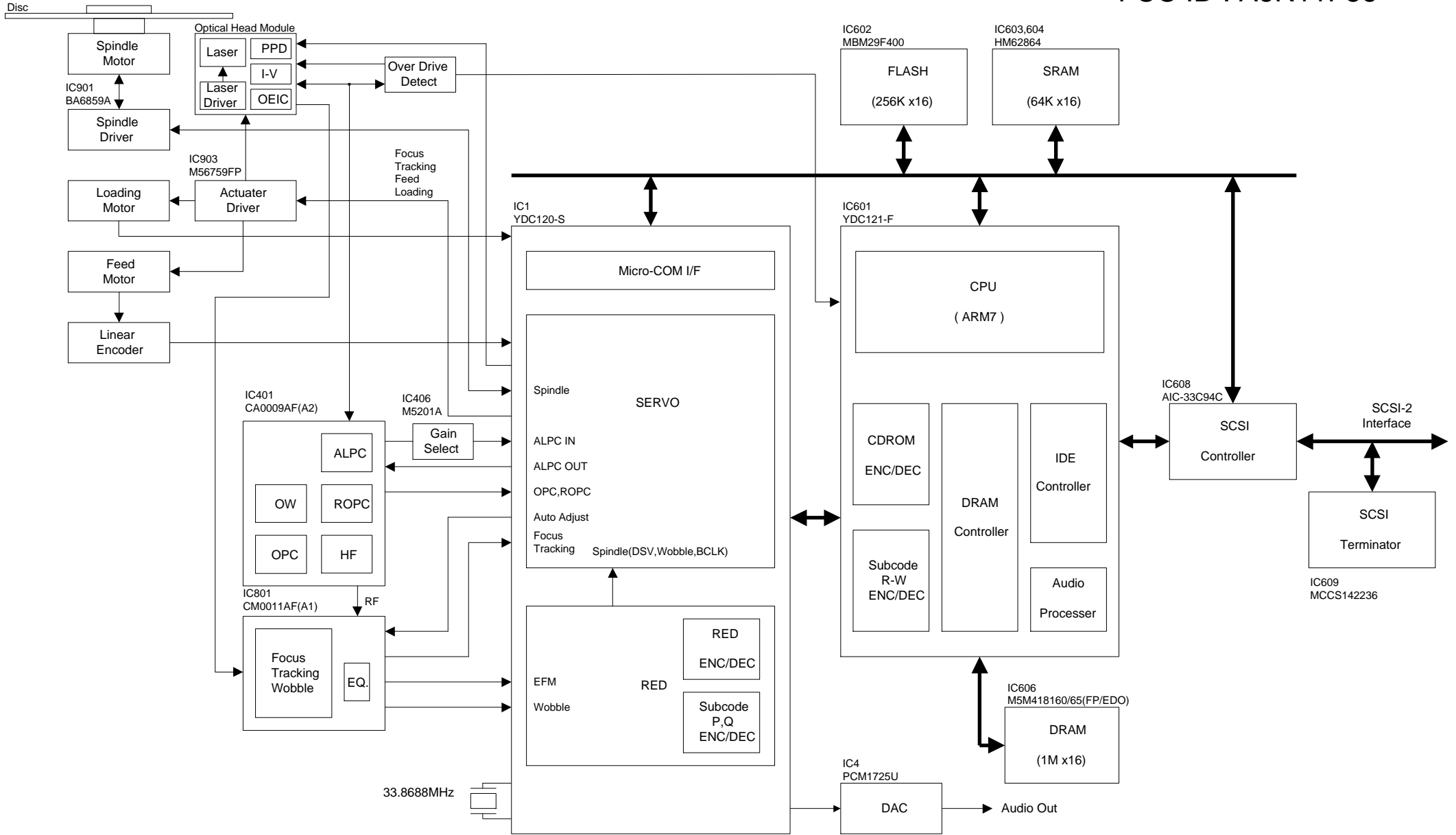
CRW4461S Series BLOCK DIAGRAM
