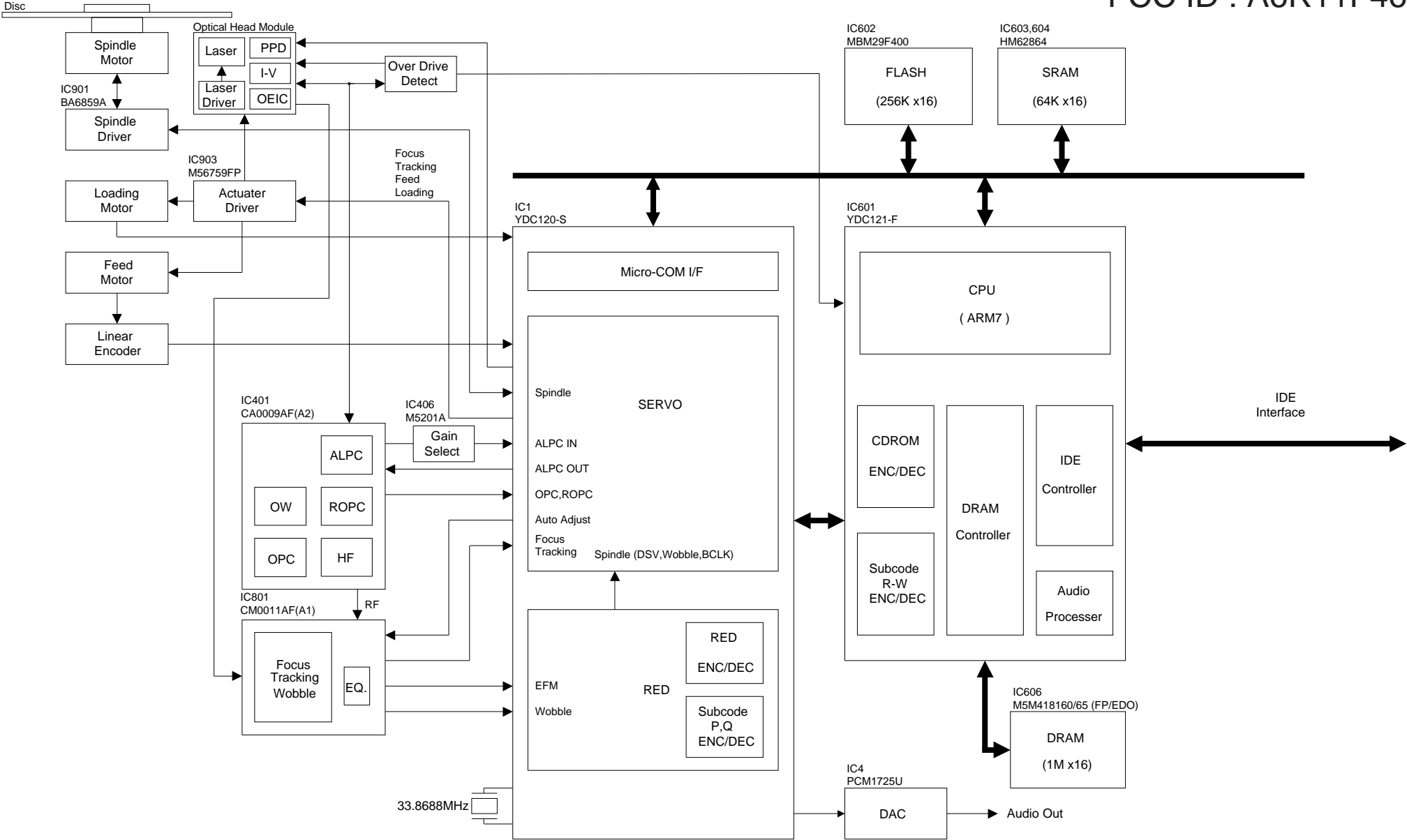
CRW4216E Series BLOCK DIAGRAM
