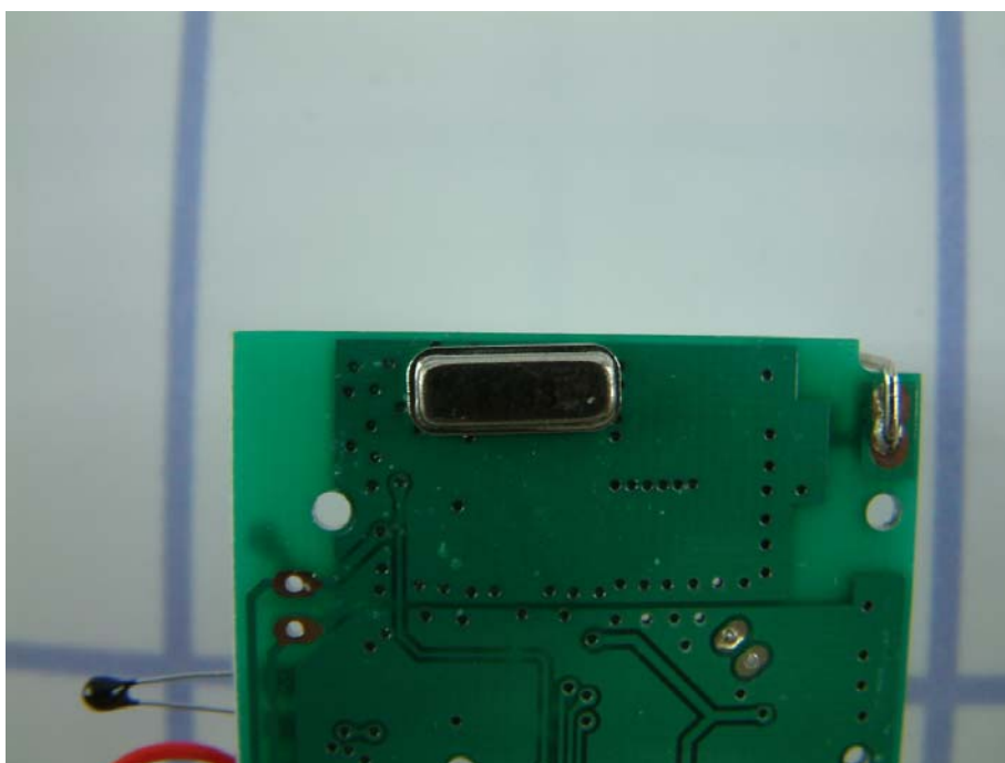
TX Oscillation view
