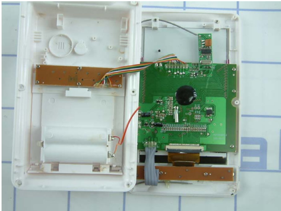
RX Internal view
