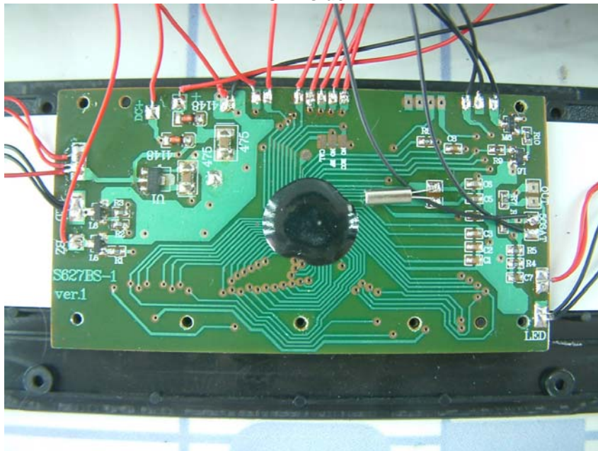
PCB2 side1
