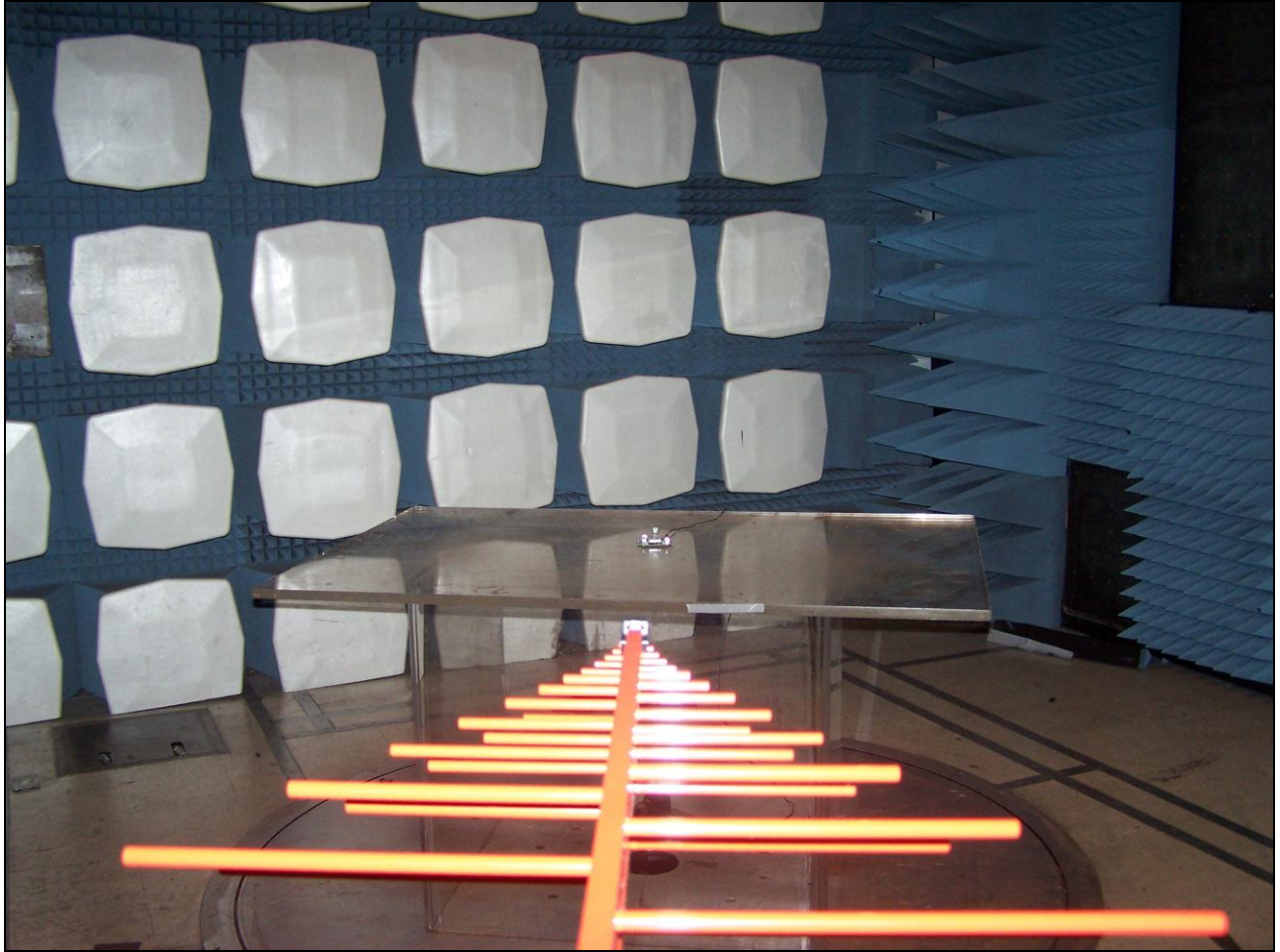
Radiated Spurious Emissions, Test Setup
