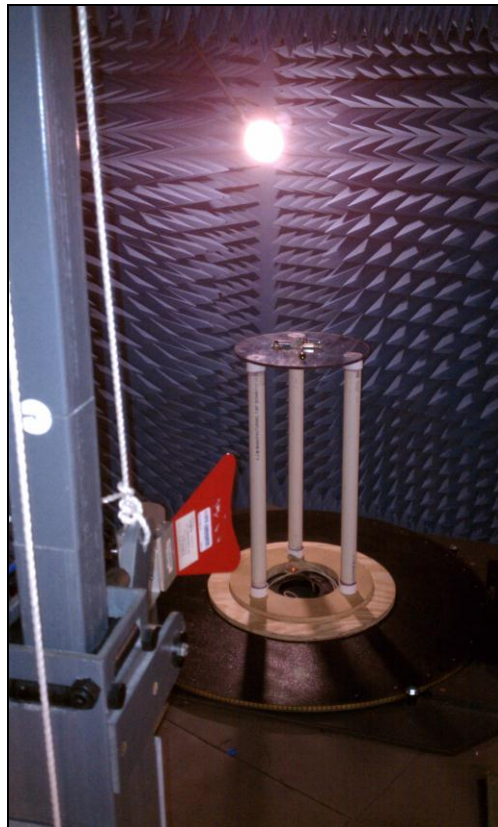
Photograph 2. Radiated Spurious Emissions, Test Setup, Above 1 GHz
