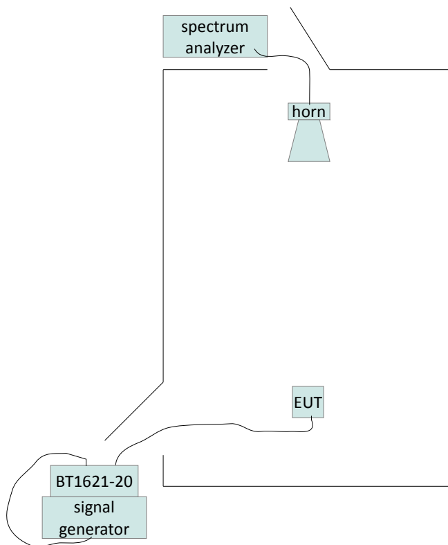
Figure 1. Diagram of test set up in anechoic chamber. Top view of anechoic chamber. Doors are closed for measurements.
