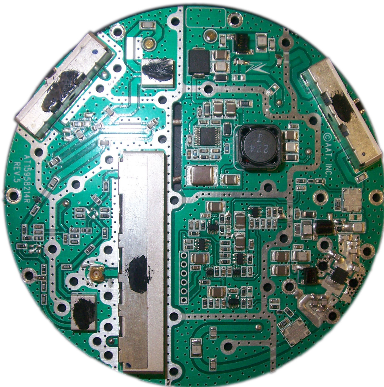
Figure 1. Top view of AT1595-82 circuit board.
