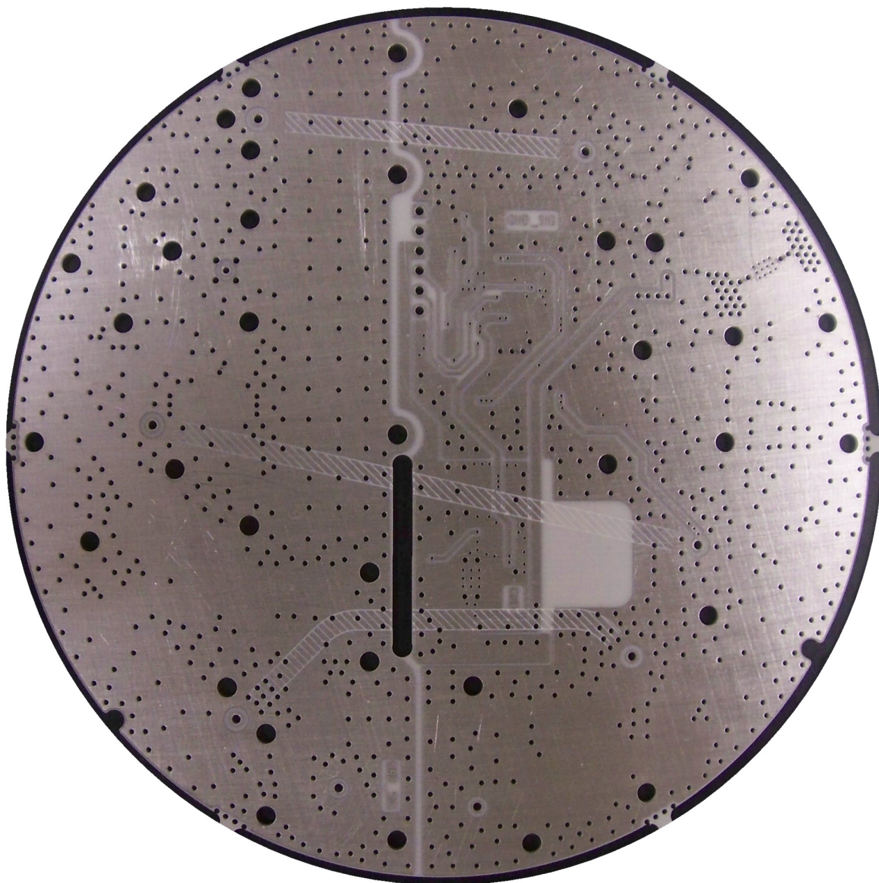
Figure 2. Bottom view of AT1595-82 circuit board.
