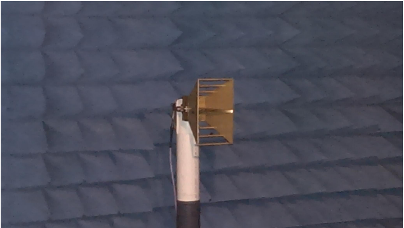
Illustration & Radiated Emissions Test Setup. Standard Gain Horn Antenna with adjustable polarization axis.
