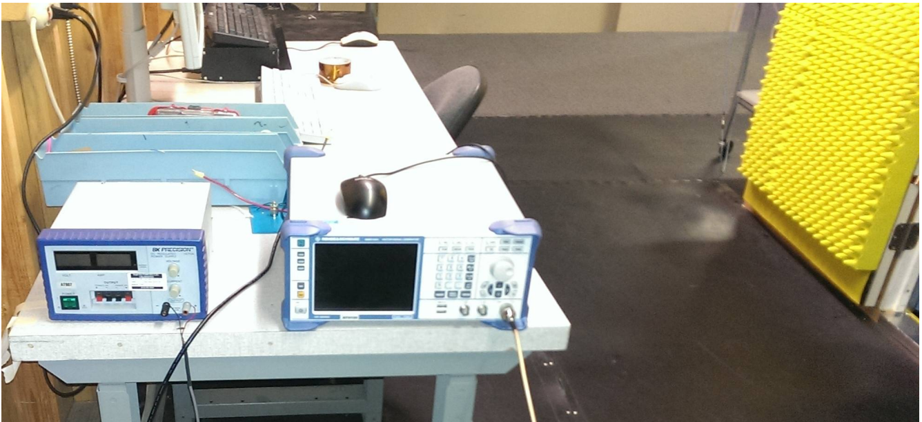
Illustration 85: Radiated Emissions Test Setup. Signal generator Source is located outside of the anechoic chamber on the E: T side.
