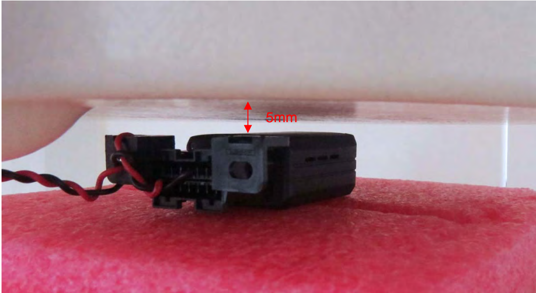
Picture 7: Back Side, the distance from handset to the bottom of the Phantom is 5mm
