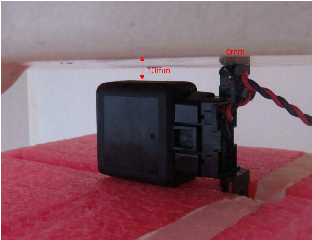
Picture 10: Right Edge, the distance from handset to the bottom of the Phantom is 0mm (13mm)
