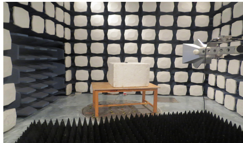
Above 1GHz
