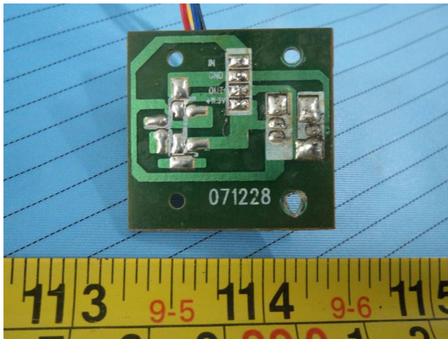
EUT – 071228 Board Bottom View
