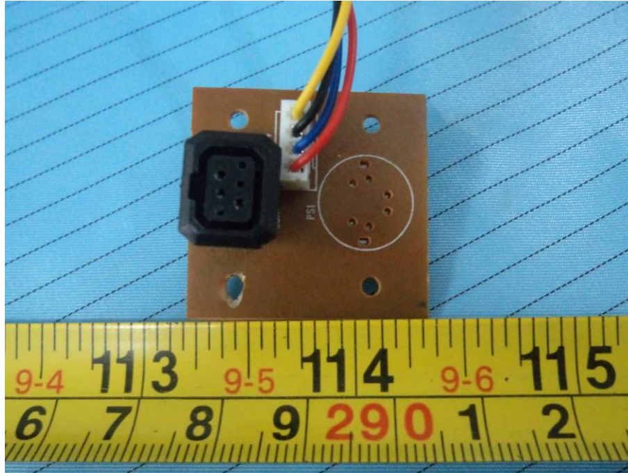
EUT – 071228 Board Top View
