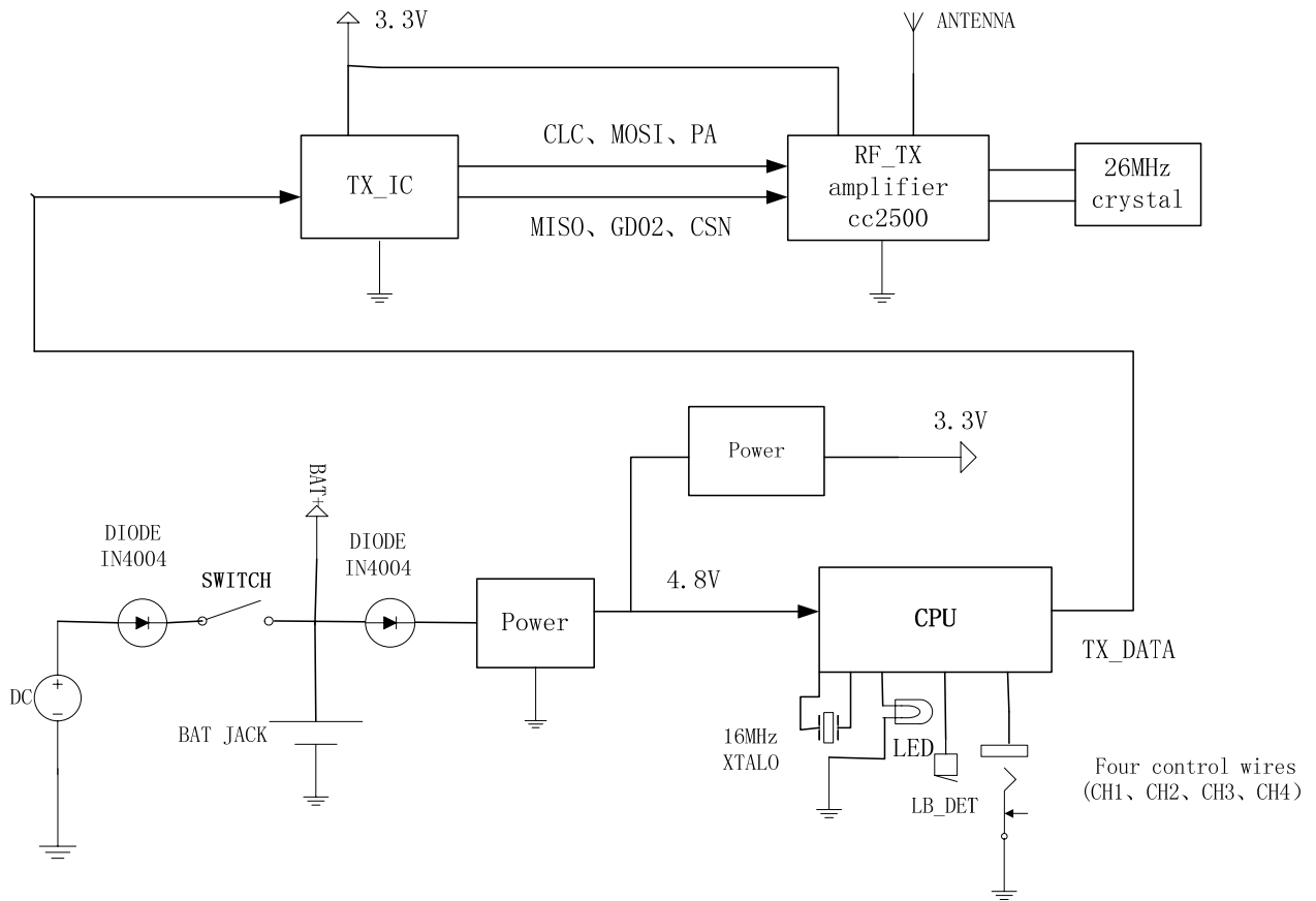
2.4G Transmitter block drawing
