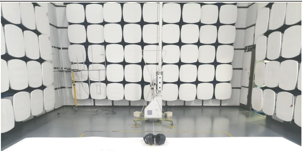
Radiated Emission
