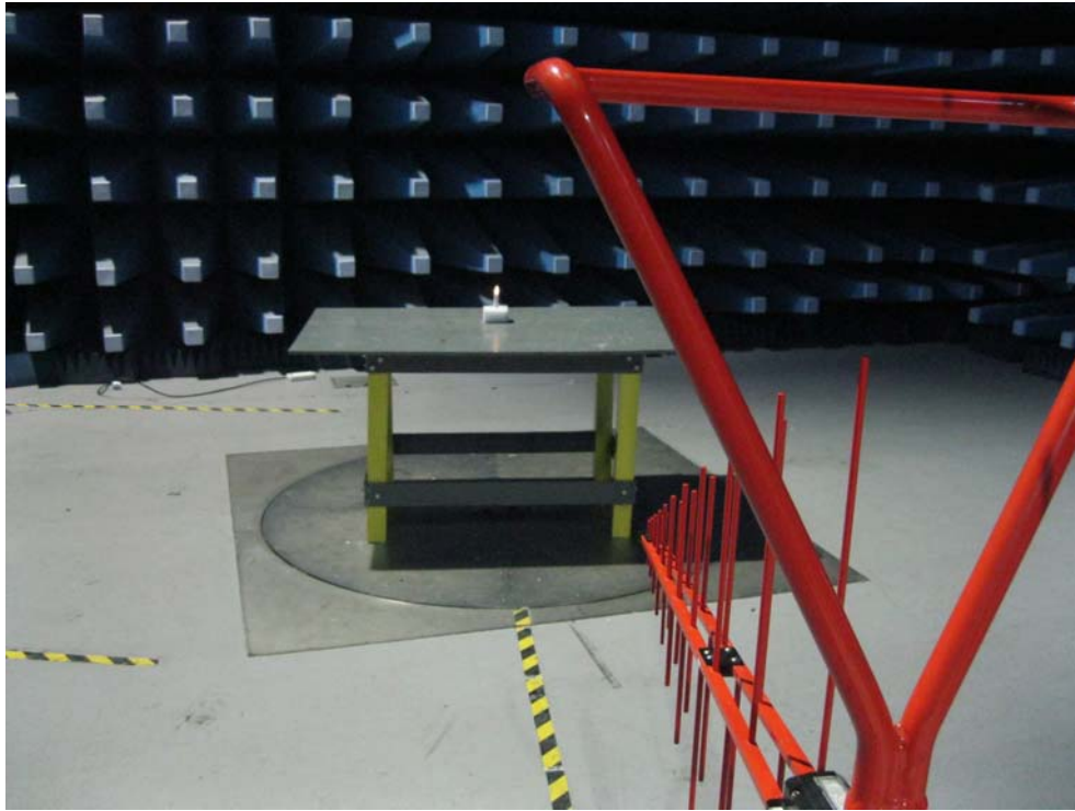
Radiated Emission Test Setup Front View
