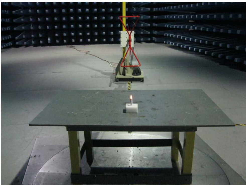
Radiated Emission Test Setup Rear View
