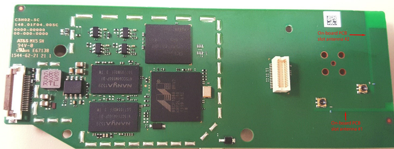
Circuit Board – Side 2 with Shield Removed
