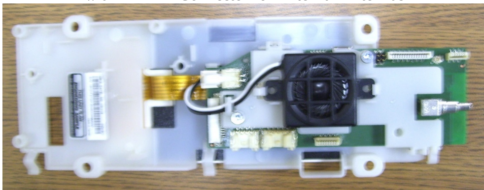
Back Side with FAKRA Connector for External Antennas
