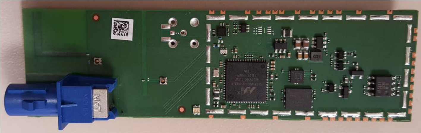
Circuit Board with External Antenna Configuration – Side 1 with Shield Removed
