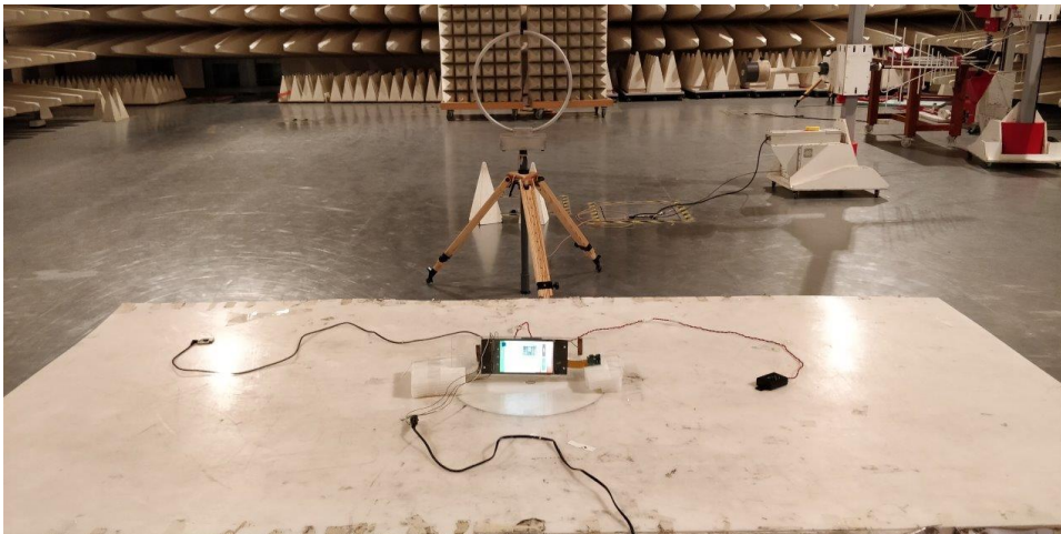
Frequency range:9kHz-30MHz
