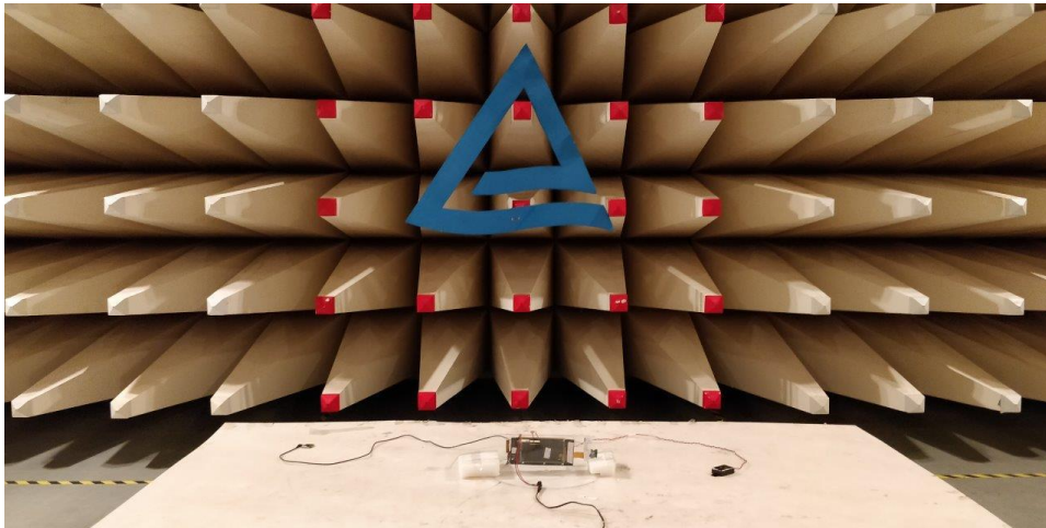
EUT Close-up
