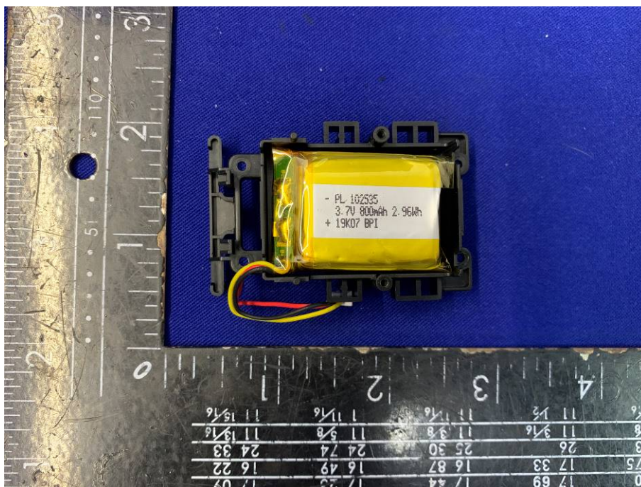
Internal battery
