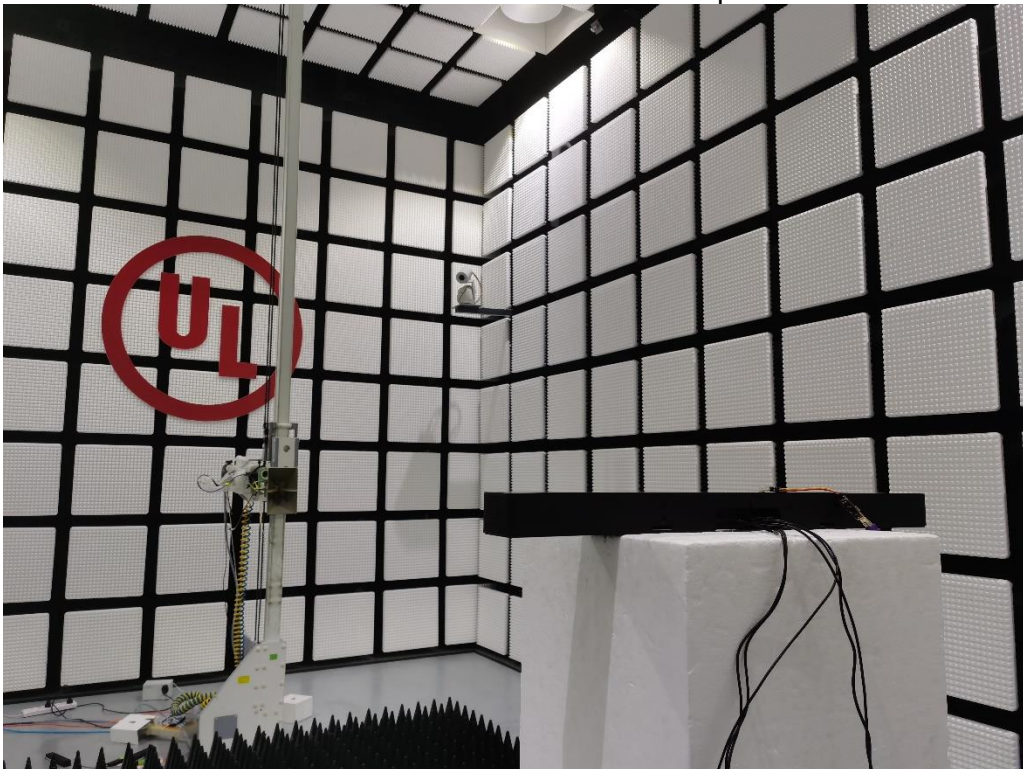
Radiated RF Measurement Setup
