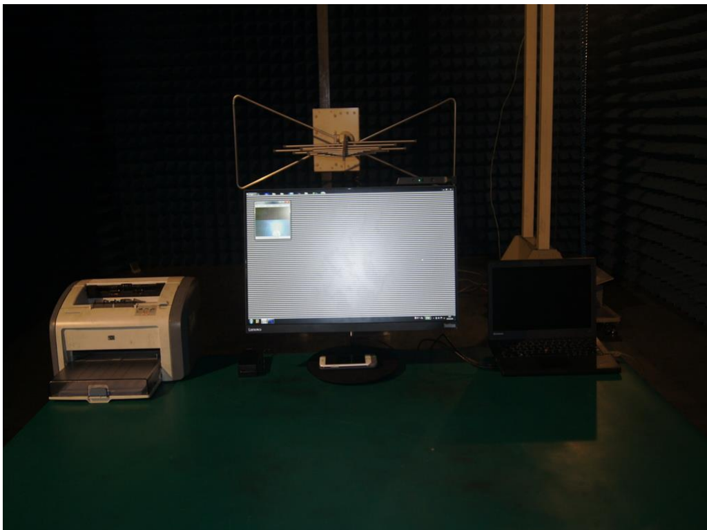
Photograph 2: Set-up for Radiated Emissions (30MHz-400MHz)
