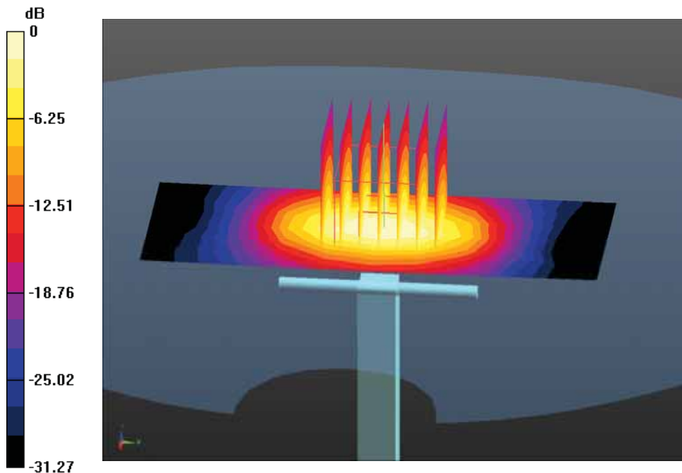
Fig. 1 – System Check
