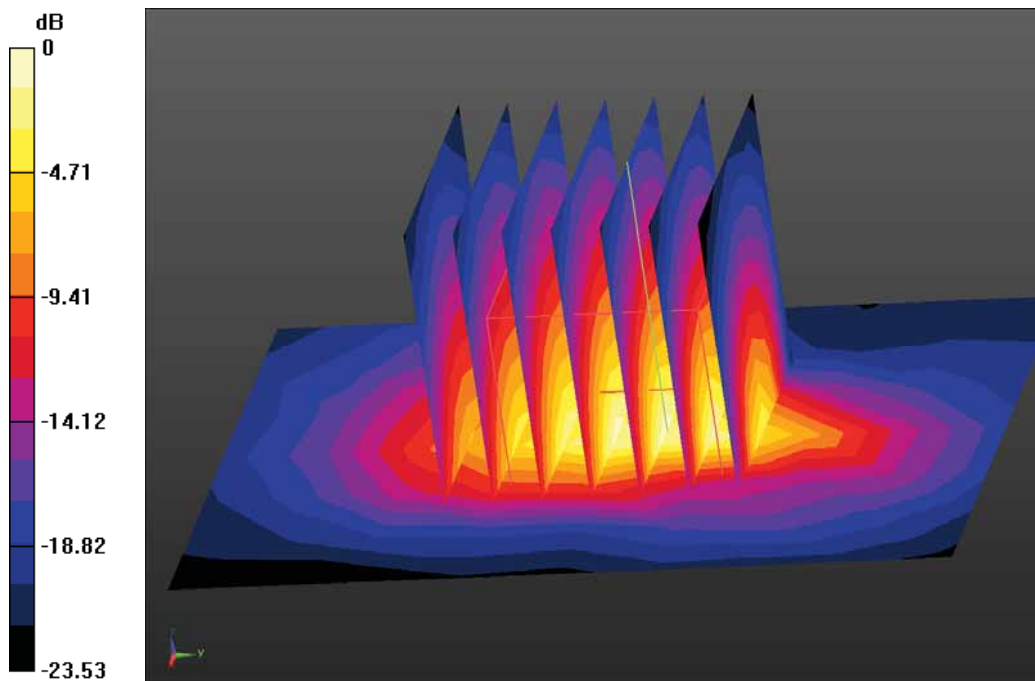
Fig. 2 - Up Side Low 802.11b Channel 1
