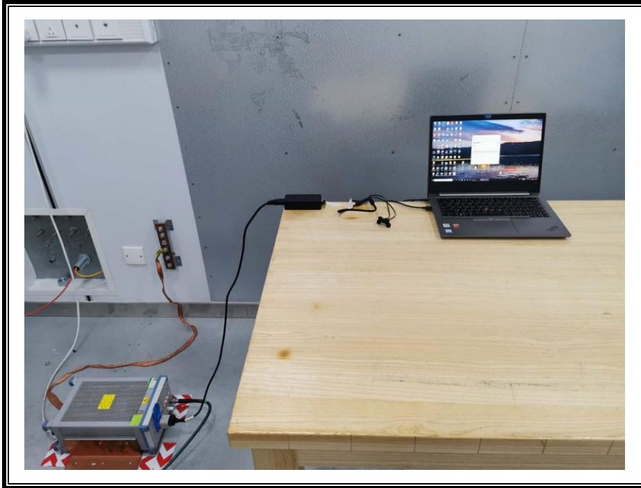
AC POWER LINE CONDUCTED EMISSIONS MEASUREMENT SETUP
