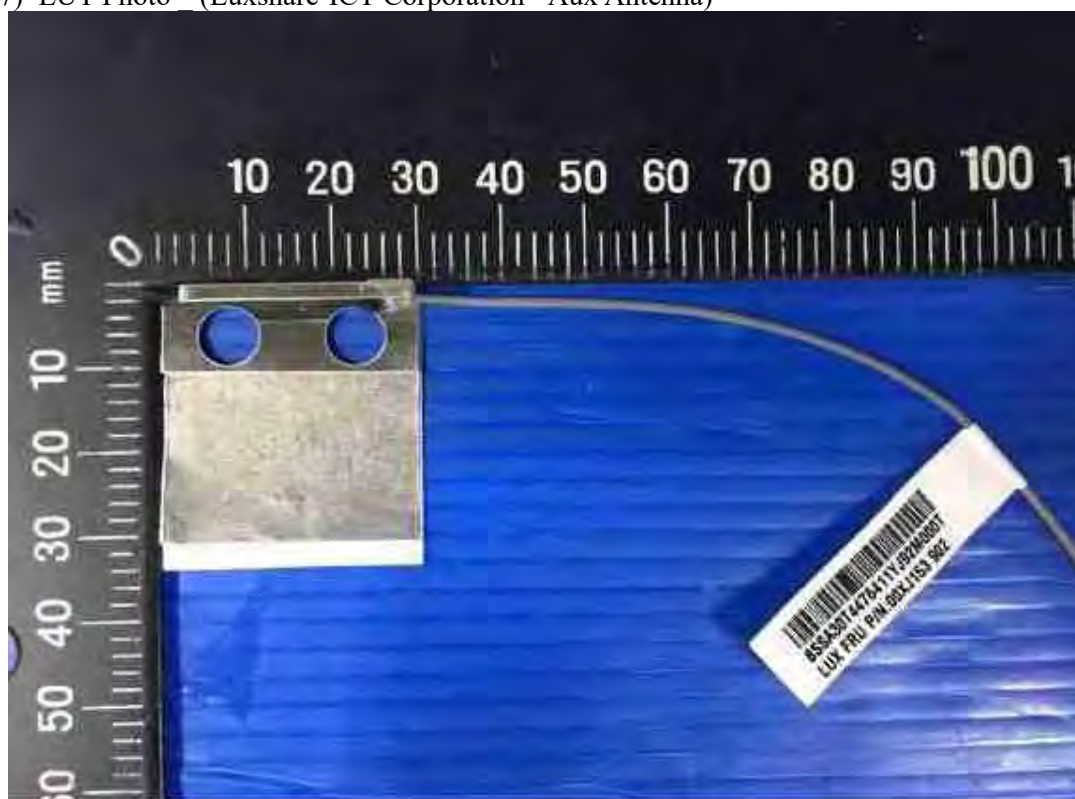
(28) EUT Photo
