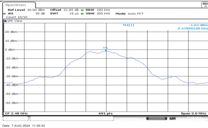
SRD 2.4G_Ant1_2480_0-Reference
