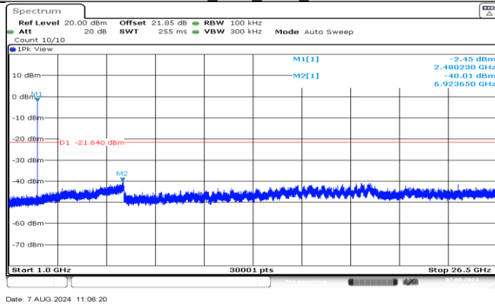
SRD 2.4G_Ant1_2480_1000-26500
