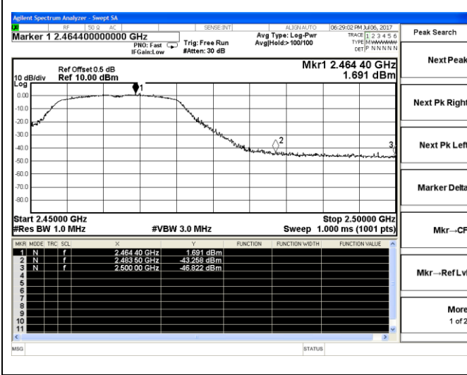
802.11n-HT20 High channel(Peak)
