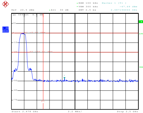
No-hopping mode
