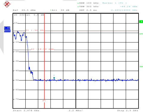
Hopping mode
