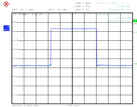
DH1/2-DH1/3-DH1
